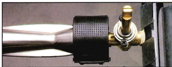
Patented Weber Spider Stopper™ Guards keep burners free of spider webs, eliminate interior burner cleaning.
